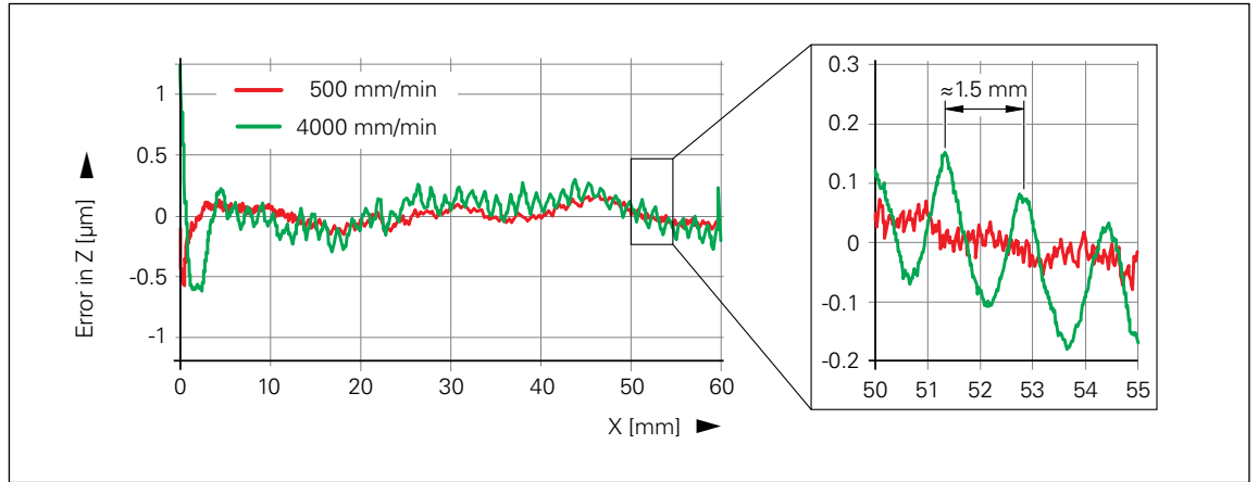
Figure 6: Measuring results for rotary encoder 1 with a 3-fold higher interpolation error
