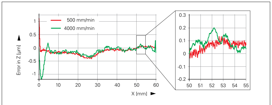
Figure 7: Measuring results with rotary encoder 2
