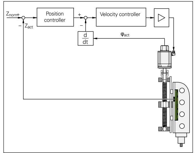
Figure 4: Schematic representation of a feed axis
