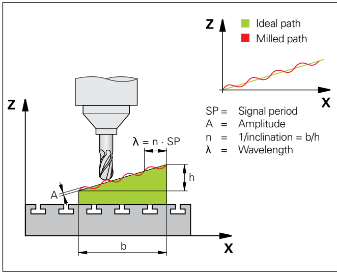
Figure 3: Illustration of interpolation error on a workpiece incline
