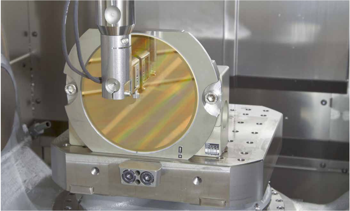
Figure 5: Measuring test setup with KGM 181 grid encoder
