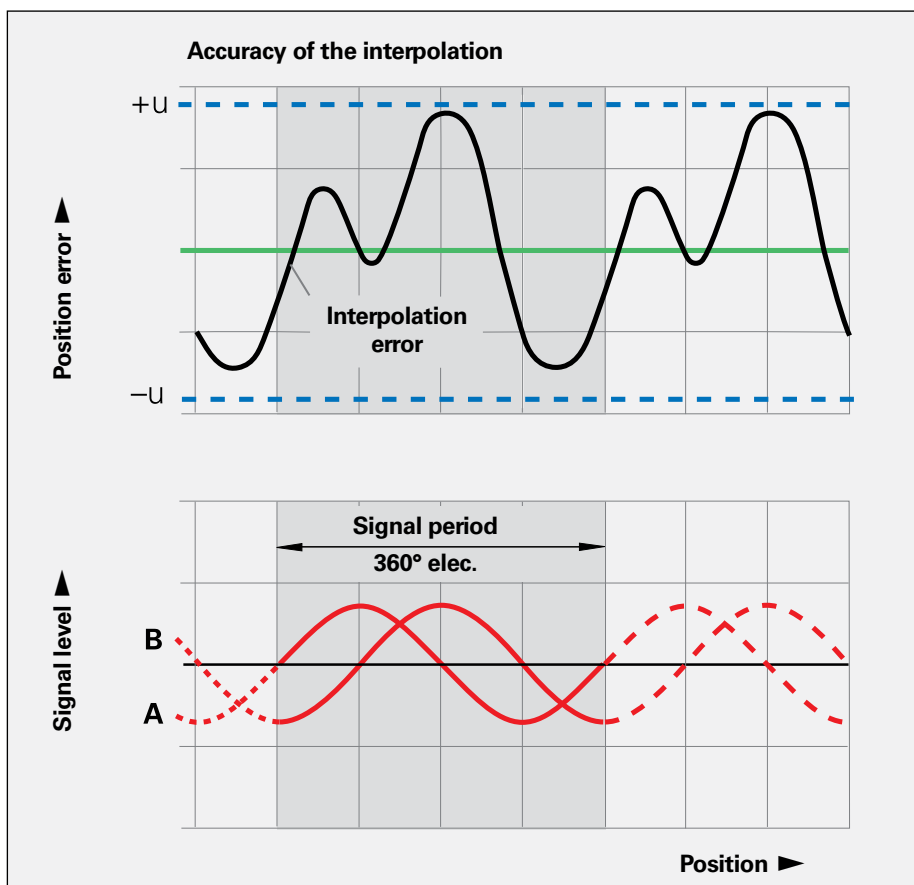
Figure 2: Position errors within one signal period (interpolation error)
